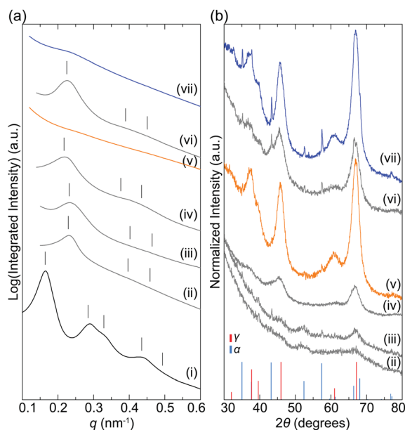
Fig. 2 (a) Azimuthally integrated SAXS, and (b) corresponding PXRD patterns of ISO- \text{Al}_2\text{O}_3 mesostructures after different heat treatments: (i) ISO- \text{Al}_2\text{O}_3 hybrid after aging at 130 °C (SAXS data only); (ii) MCA-C-1000-3 h; (iii) MCA-C-1100-3 h; (iv) MCA-C-1200-3 h; (v) MCA-CASH-1200-3 h; (vi) MCA-C-1200-6 h; (vii) MCA-CASH-1200-6 h. Tick marks in (a) indicate the expected SAXS reflections for a hexagonal ( p6mm ) lattice. PXRD peak markings and relative intensities for \gamma\text{-Al}_2\text{O}_3 (red, PDF 00-010-0425) and \alpha\text{-Al}_2\text{O}_3 (sky blue, PDF 04-004-2852) are shown in (b). The data sets in (a) and (b) are offset vertically for clarity.
