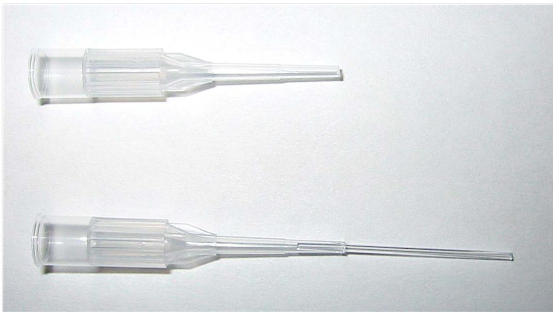
Figure 4.38: Modified 10 \mu\text{L} Rainin LTS pipet tips for use with polycarbonate capillaries.
