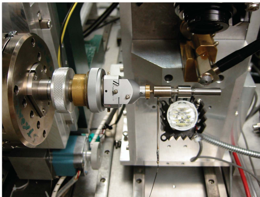
B: Beryllium cell mounted on CHESS station F1 goniometer
