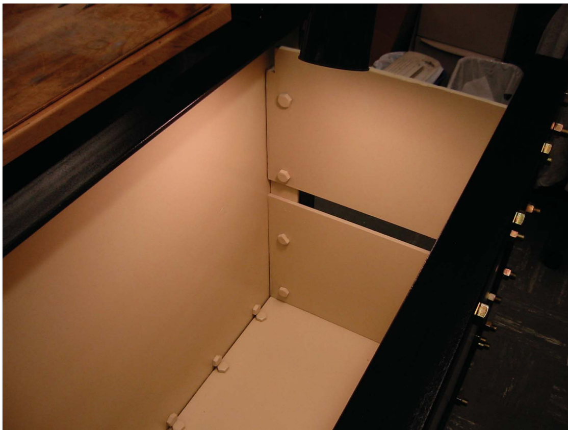
Figure 4.9: View of gas exit port (plates G and H in figure 4.7) from inside the high-pressure cryocooling safety enclosure.
