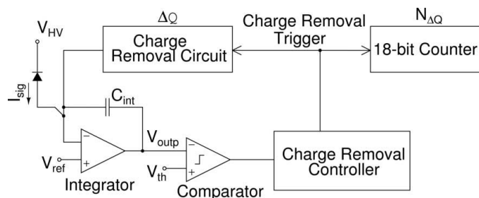
Figure 1 A high-level schematic of the pixel architecture. Photo-charge ( I_{sig} ) from the reverse-biased diode is integrated across C_{int} . When the comparator senses a near-to-overflow condition, a charge removal operation, which increments a count in the 18-bit counter, is triggered. The pixel output at the end of an exposure is the combination of the digital counts ( N_{\Delta Q} ) and the analog residual ( V_{outp} ) (Schuette, 2008).
