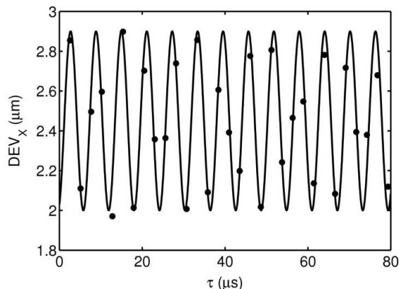
Figure 11 Fluctuations of the CHESG G3 beam horizontal position at fast time scales with a superimposed oscillation (solid line) at 163 kHz.
